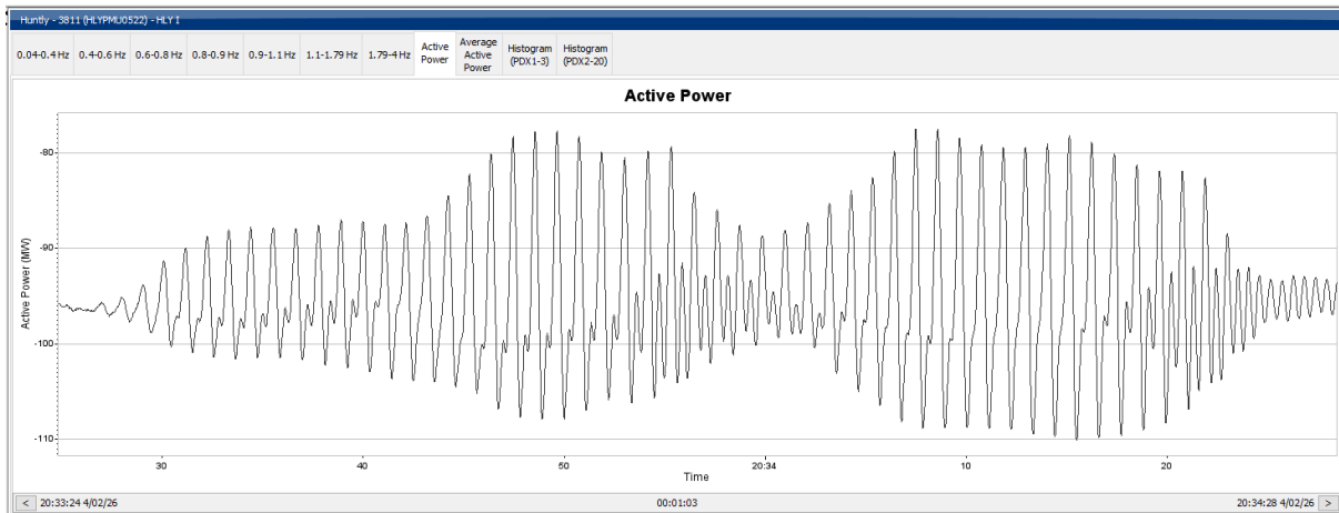
Huntly PMU (HLY_SFD circuit) Power recording during the oscillation period
